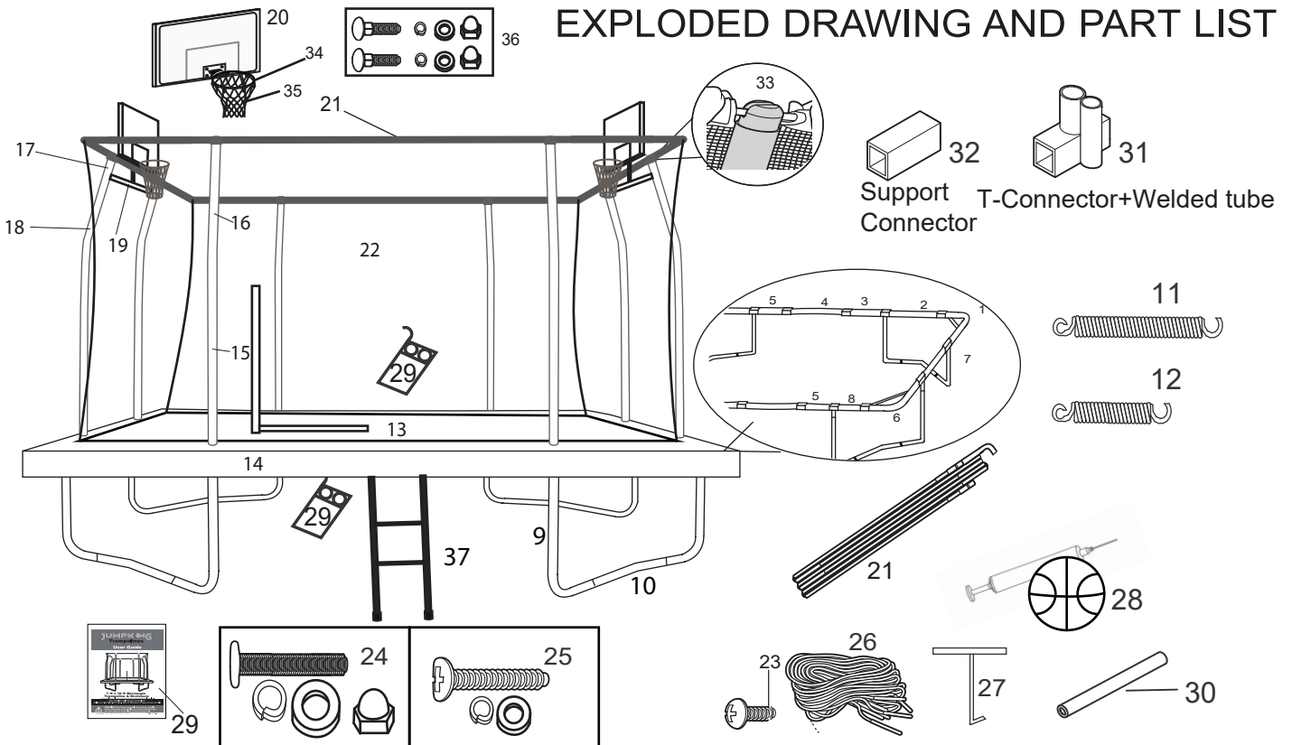
Trampoline Assembly Parts Listing
